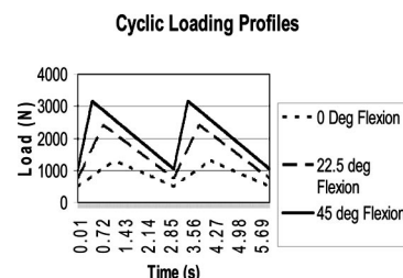
Figure 3. Loading profiles for simulated lifting of 9-kg load in 0°, 22.5°, and 45° of torso flexion.
