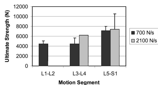
Figure 5. Ultimate strength for specimens lasting maximum number of loading cycles. Lack of a standard deviation bar indicates only one specimen was tested in this condition.
