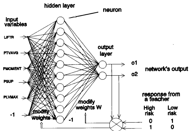
Figure 3 The architecture of the neural network used for system training purposes
